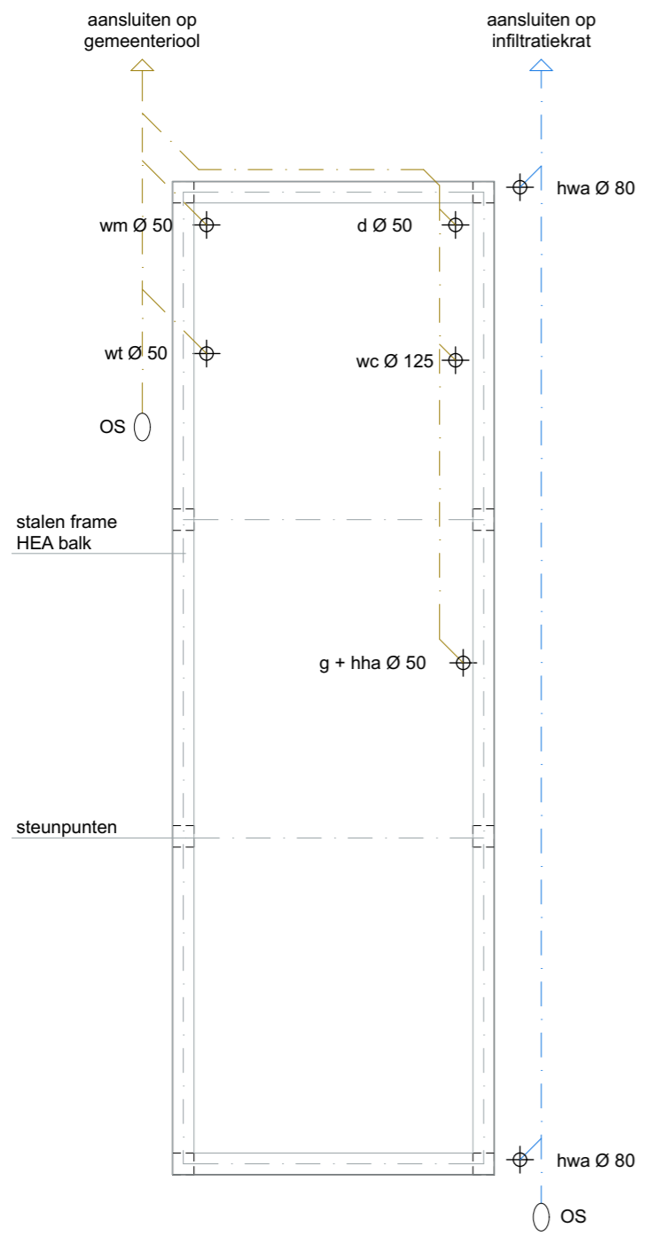
fundering/riolering
